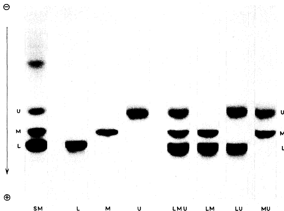
Fig. 2. Electrophoretal analysis of rat brain myelin proteins. Protein fractions L, M, and U were isolated from crude myelin by SDS extraction and subsequent separation on a preparative polyacrylamide gel column. For details see fig. 1.
